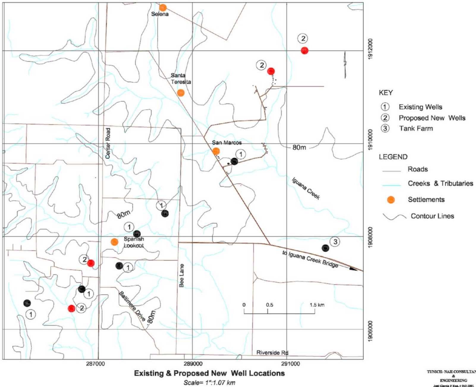
Fig. 1.1 Existing and Proposed New Well Locations for BNE
